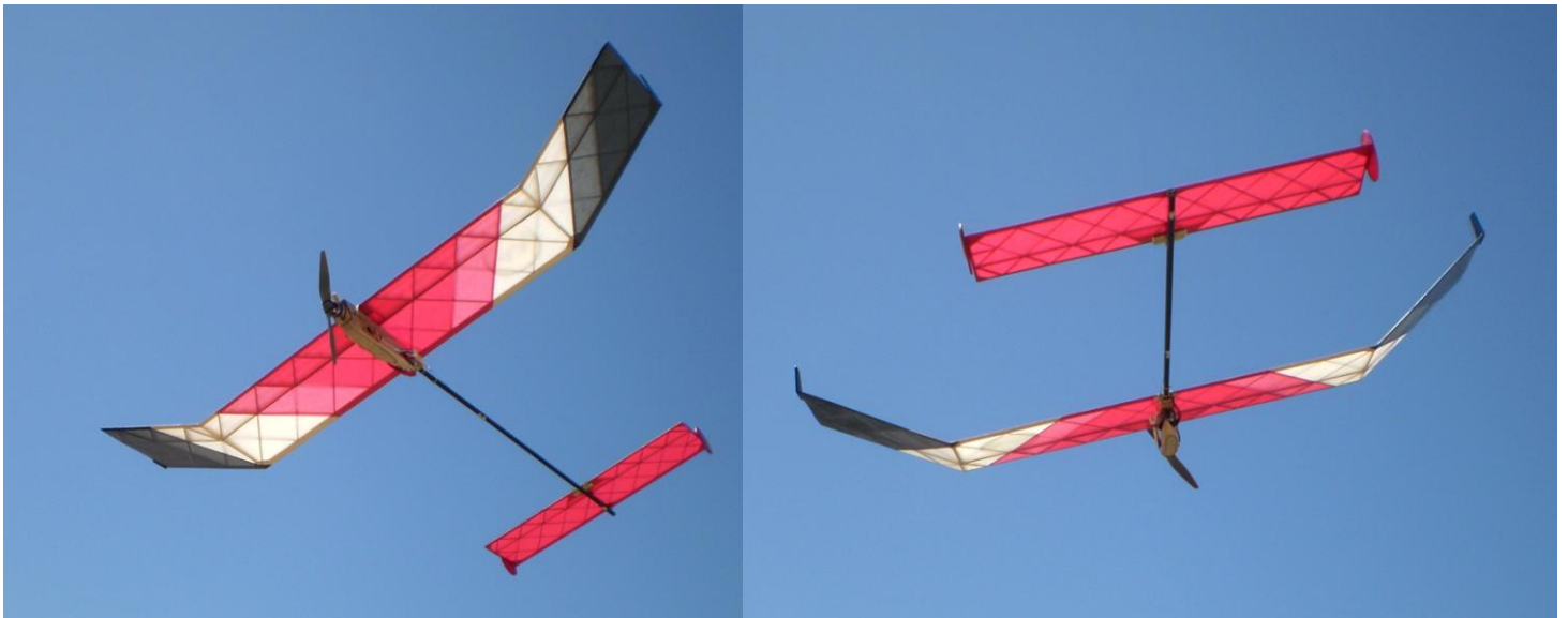
Apache II Prototype T-1-the this is the fourth version in the series of development models flown in late 2014 and throughout 2015 and 99% representative of the pending kit release later this year-try one!
