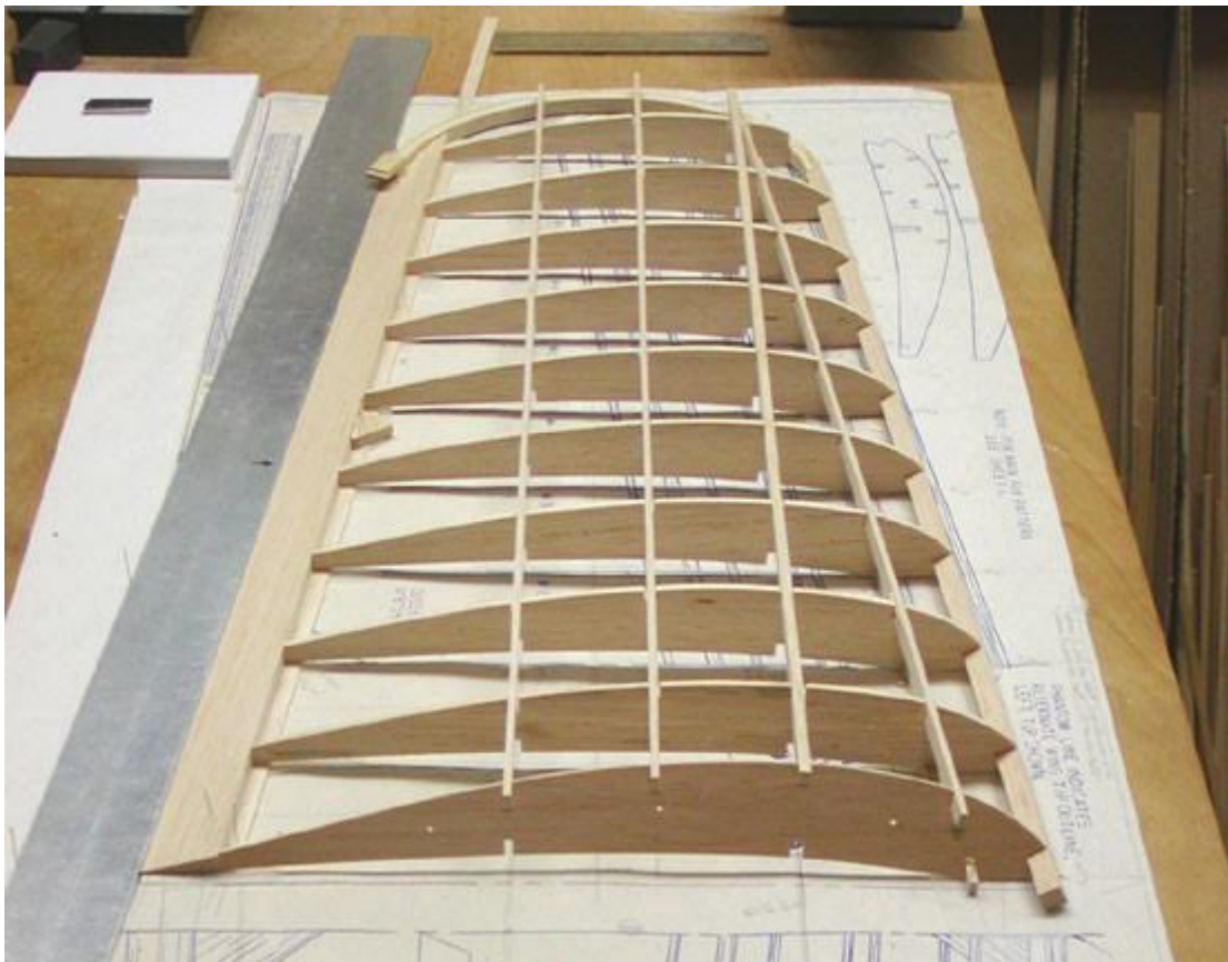
This shows all three top spars installed on the left wing tip panel. Notice how straight they are. :O)
