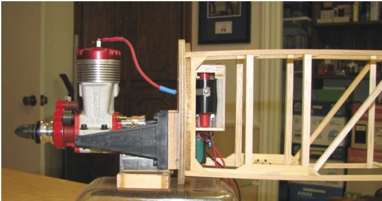
Frontal view from the left side showing high tension lead routing, which will be mostly under the cowl.
