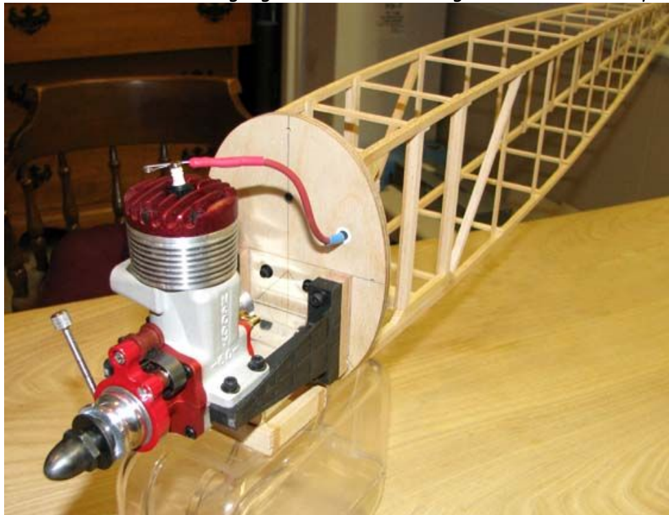
Frontal view from the left side showing high tension lead routing, which will be mostly under the cowl.
