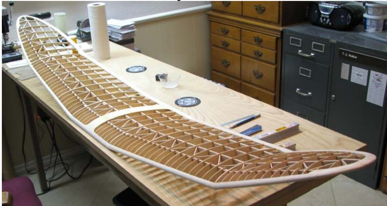
Wing Structure
